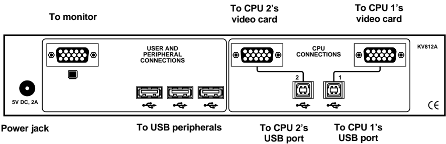
Figure 2-2. The rear panel of the 2-port ServSwitch USB (KV812A).
